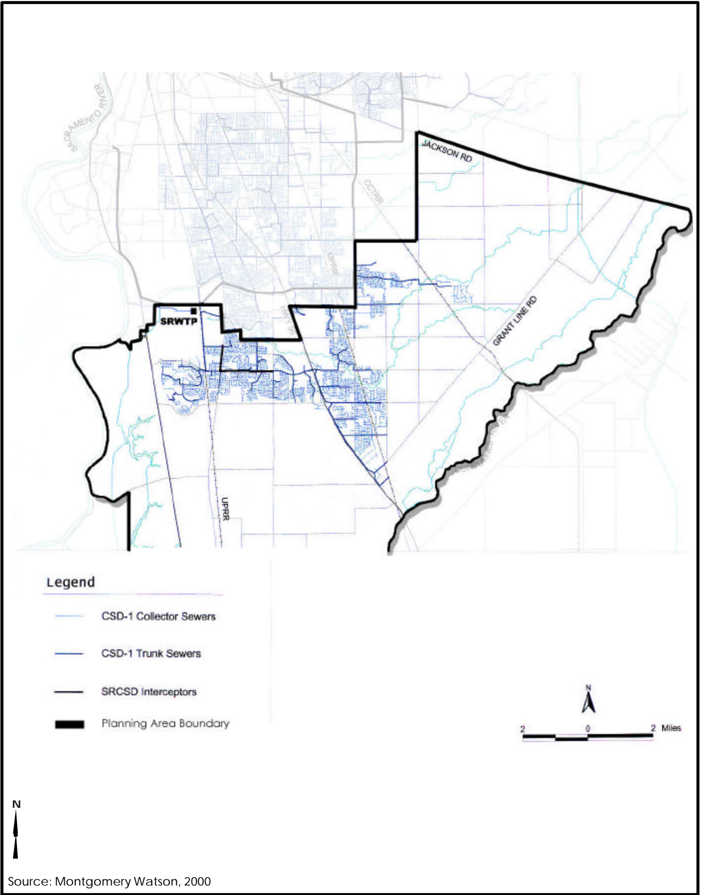
Figure 11-3 Existing CSD-1 Sewer System
