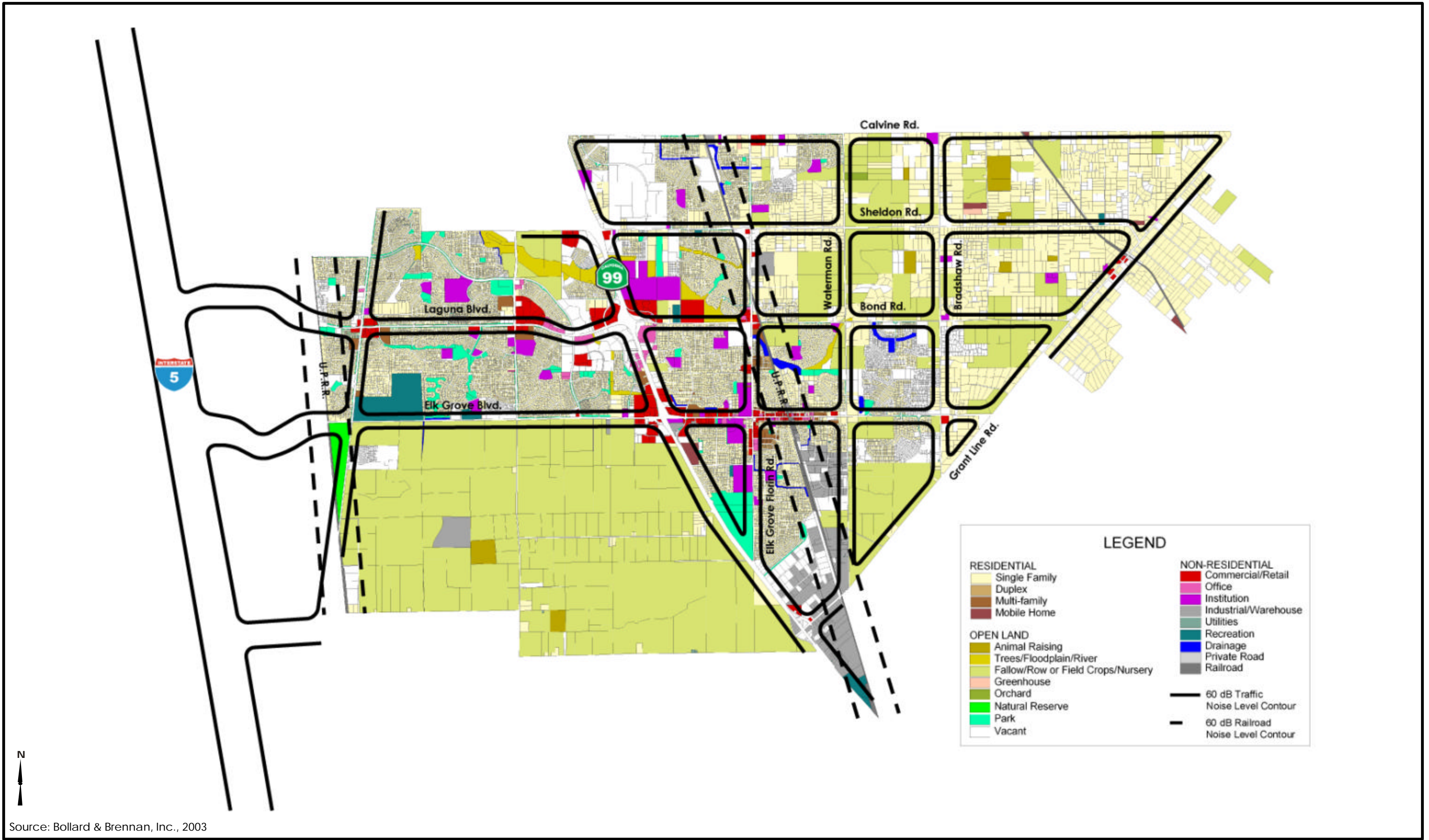
Figure 4-1 Existing Traffic Noise Contours
